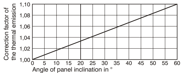
Fig.9 Corrective coefficient of emissions for inclined panels
