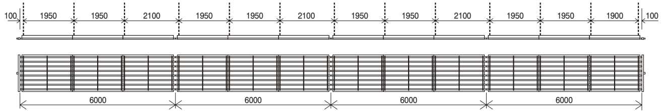
Fig.33 Example of distance between suspension points with modules of 6 metres
