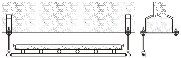
Fig.42 Example of brackets with roller for panels transversal to roof tiles
