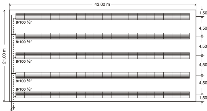
Fig.14 Example of ECOPAN panels in warehouse with average height of 5.5 m and parallel panels on greater side
