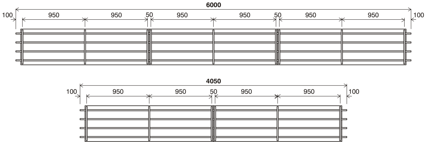
Fig.2 Suspension brackets (mm)
