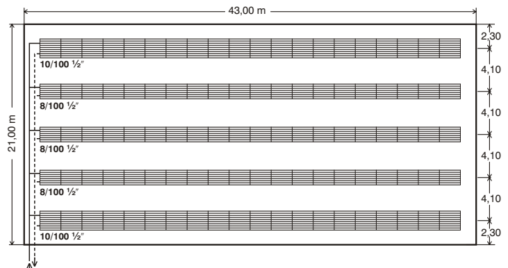
Fig.15 Example of ECOPAN panels in warehouse with average height of 5.5 m and parallel panels on greater side
