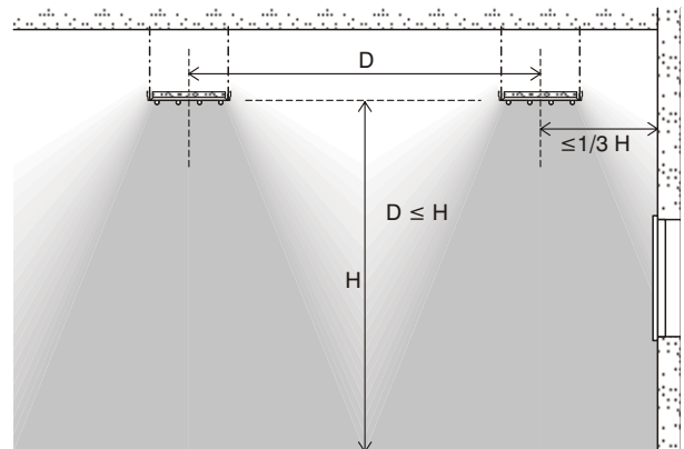
Fig.10 Distance between radiant panels
