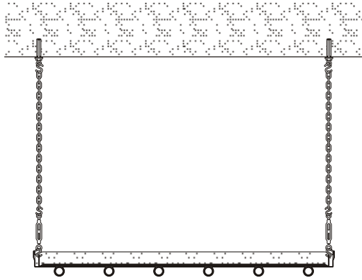
Fig.38 Example of brackets with chains
